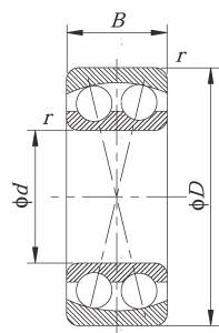
Cylindrical bore
