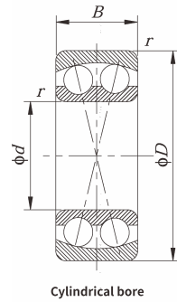
Cylindrical bore
