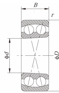
Tapered bore
