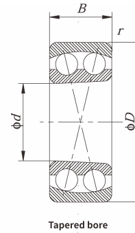
Tapered bore
