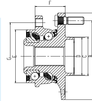
Gen 3 drive wheel bearing
