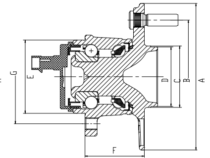
Gen 3 non-drive wheel bearing
